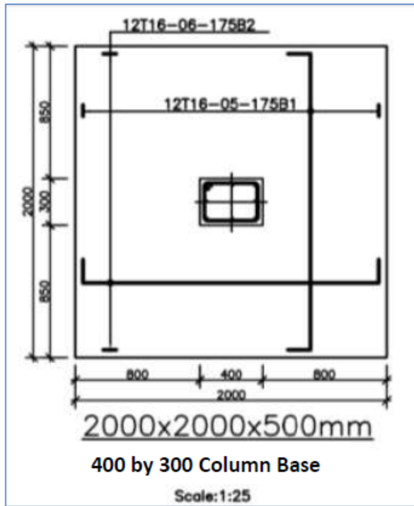
Figure 6: Typical column base design
