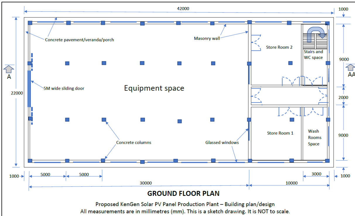
Figure 2: Floor plan of the production factory building.
