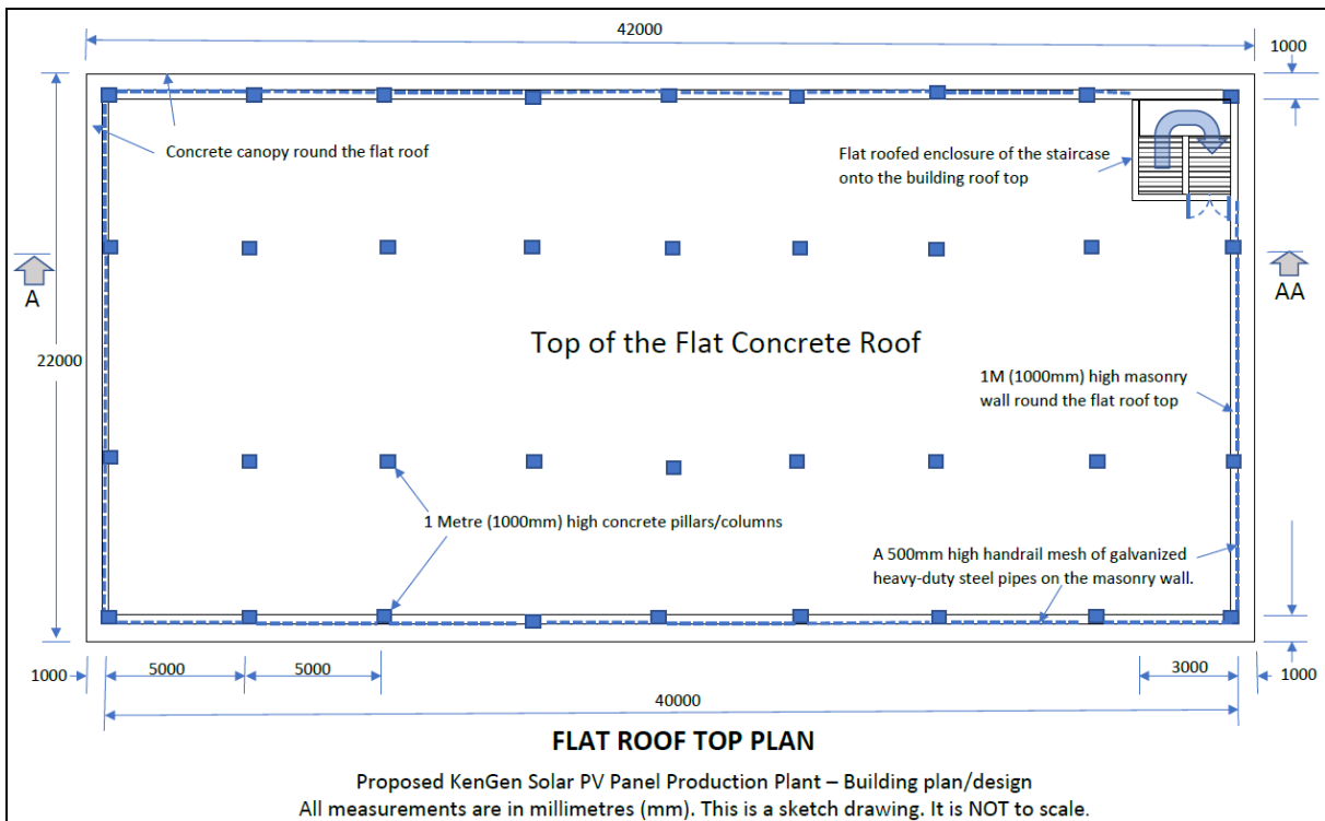
Figure 3: Flat Roof top plan
