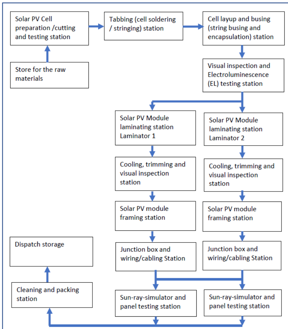
Figure 9: Illustration of flow of activities in the Solar PV panel production plant
