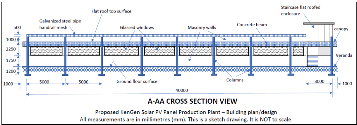
Figure 4: The cross-section view of the building
