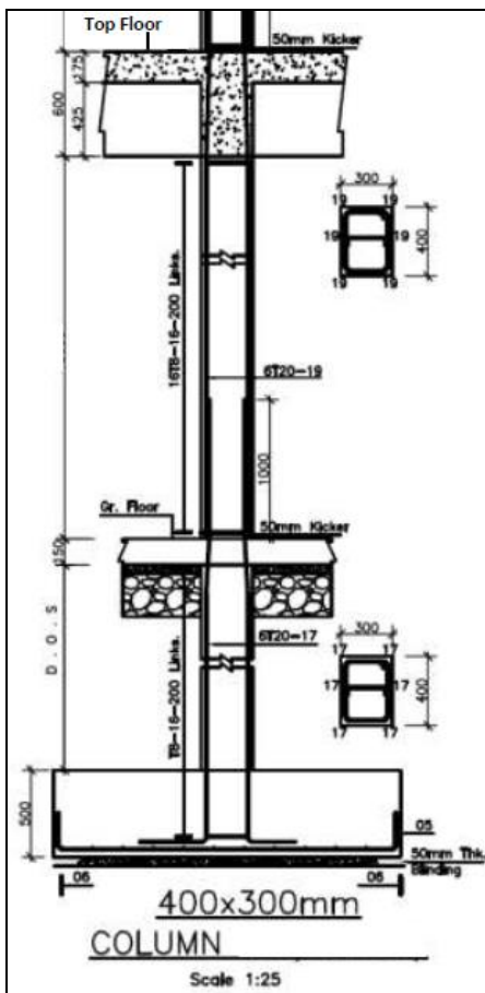
Figure 5: Typical column details
