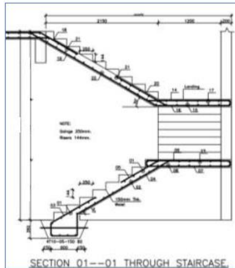
Figure 7: Typical walls' foundation details Figure 8: Staircase details
